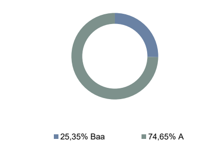
Ratings distribution
