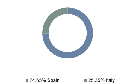
Geographic distribution
