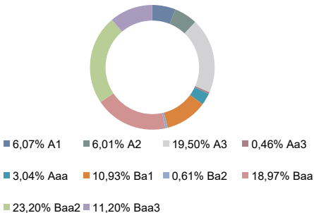
Ratings distribution
